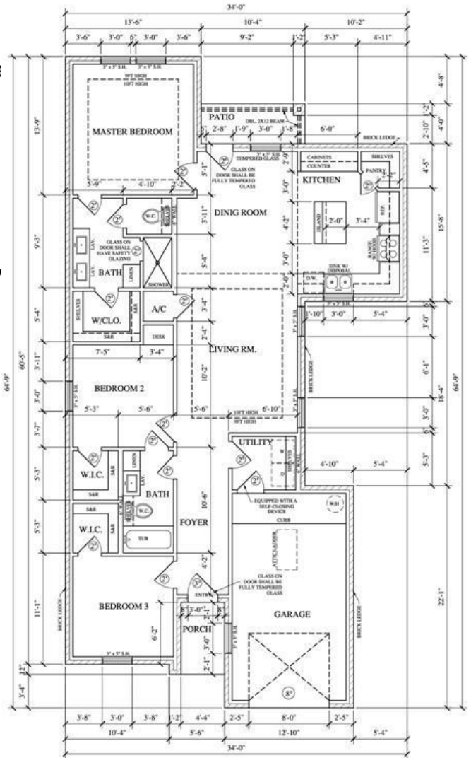
FLOOR PLAN SCALE: 1/4"=1'-0"
